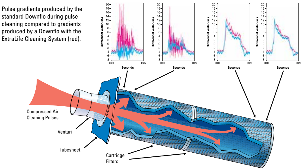
DOWNFLO PULSE PRESSURE GRADIENTS
