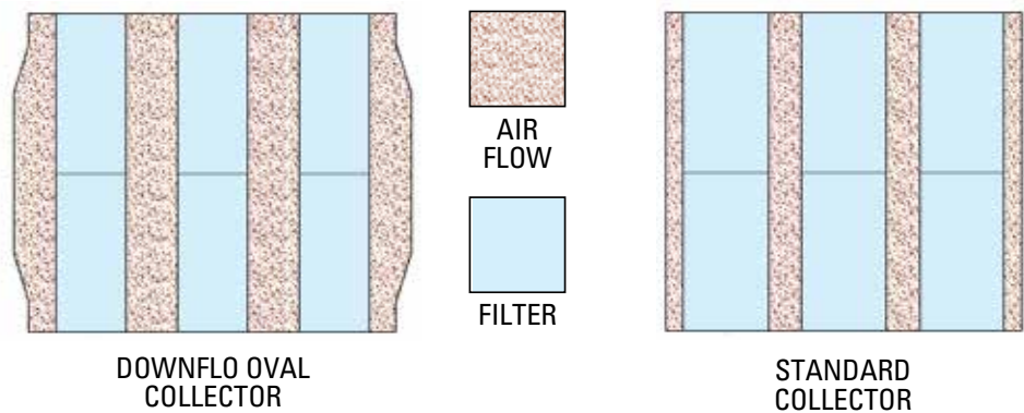
CROSS-SECTIONAL AREAS
